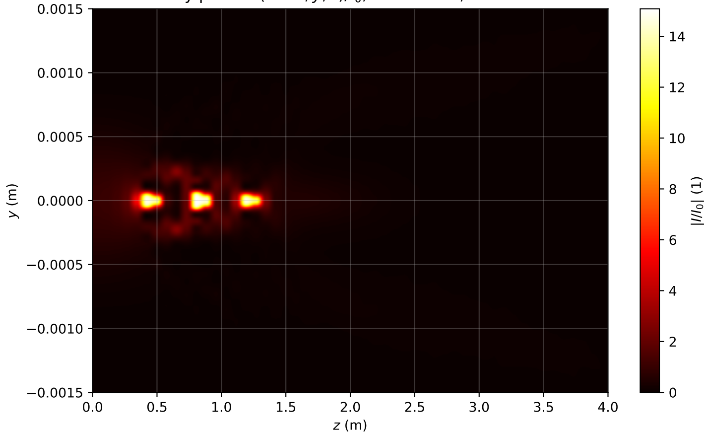
Intensity profile I(x=0, y, z)/I_0 , Pin=7.5Pcr, artificial time
